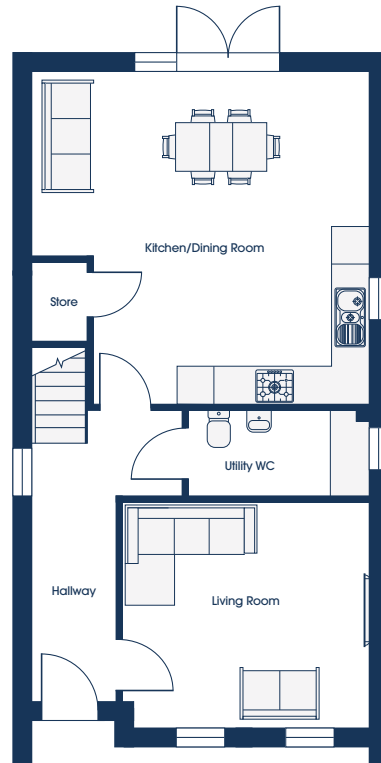
STANDARD FLOORPLAN
