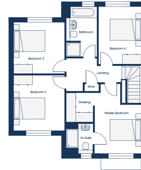
STANDARD FLOORPLAN
